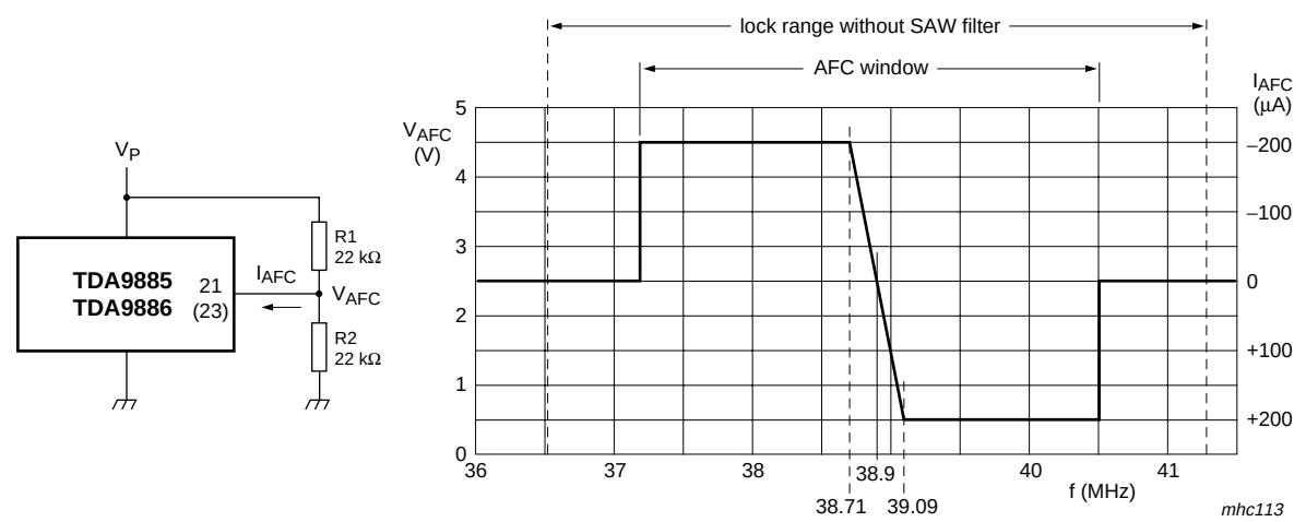
Fig 12. Typical analog AFC characteristic
