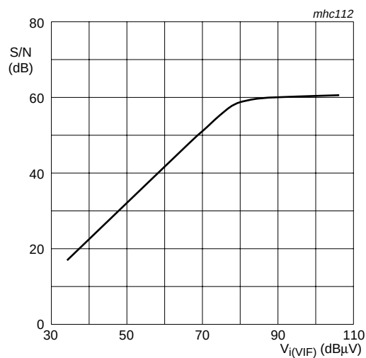
Fig 13. Typical signal-to-noise ratio as a function of VIF input voltage
